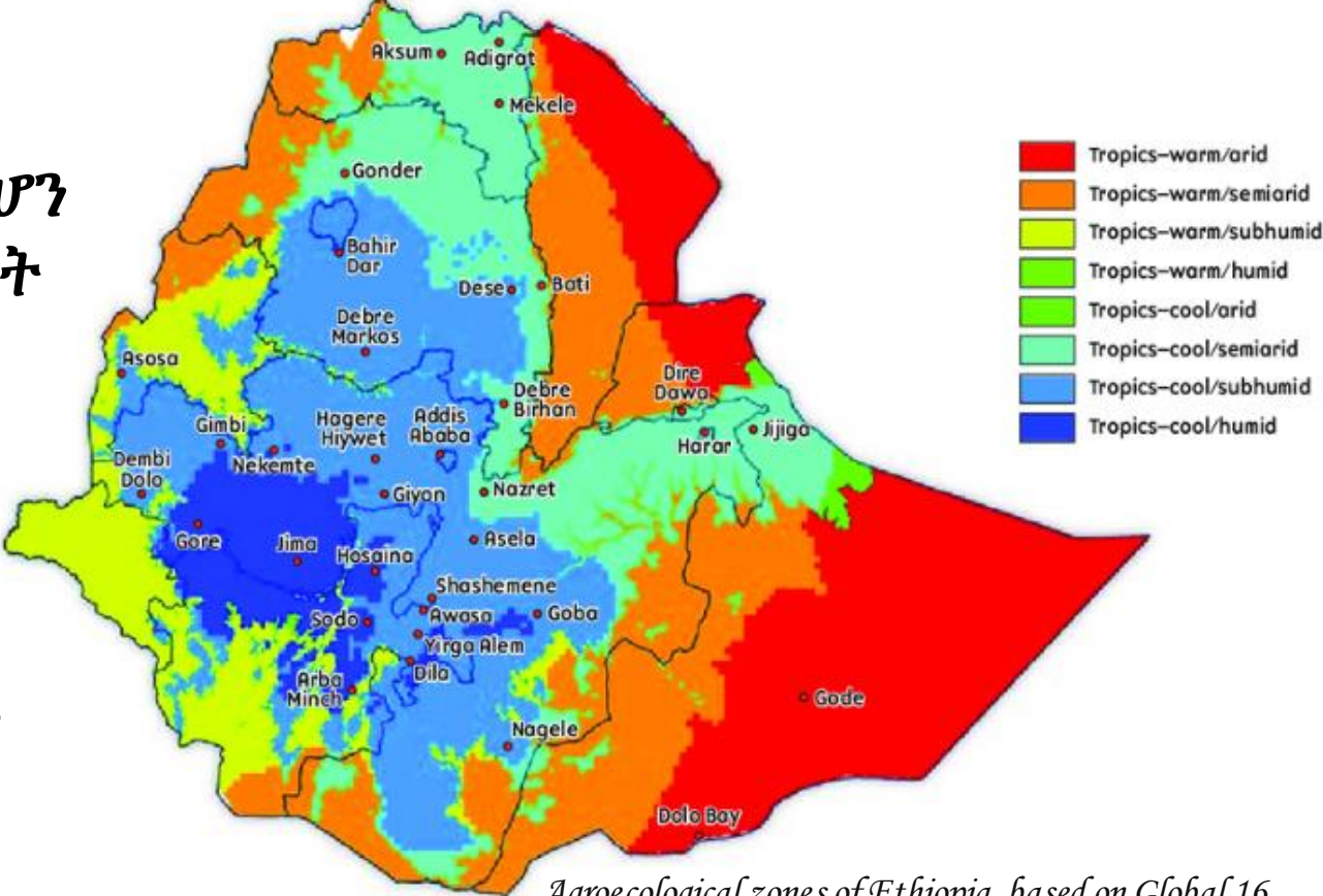
Agroecological zones of Ethiopia, based on Global 16 Class classification system (Sebastian 2009).
