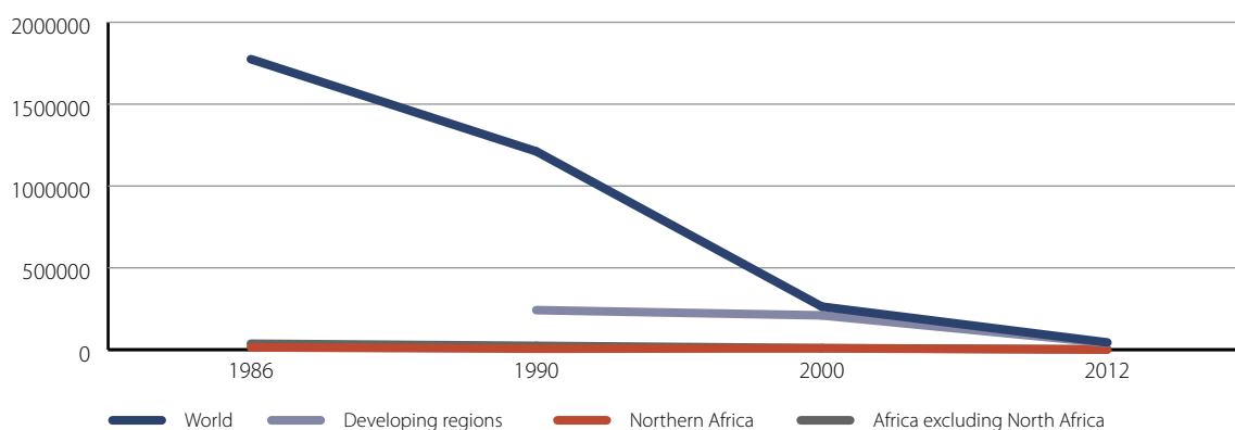
Figure 7.1 Consumption of ozone-depleting substances (1,000 metric tonnes)
